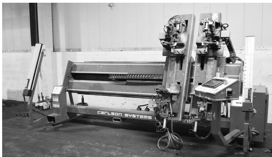
Carlson System Eng. #D2071F Four Corner Auto Window/Door Screwing System
