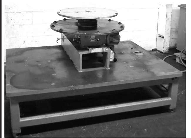
Camco 36" Rotary Index Table, 12 Position
