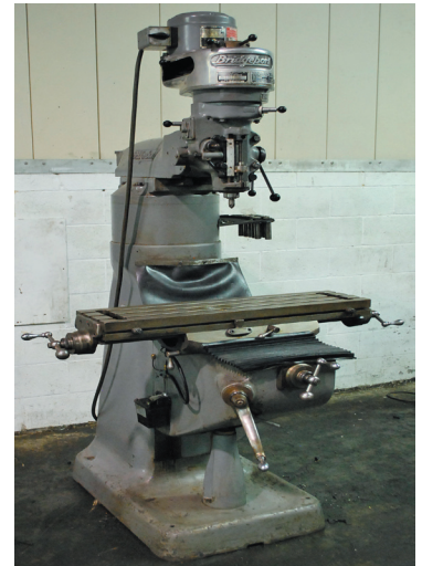
Bridgeport 1 HP Vertical Mill
