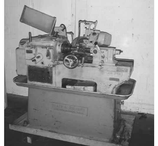
Pratt & Whitney #C 4 1/2 x 12 Thread Mill CB 1259 $1,950
