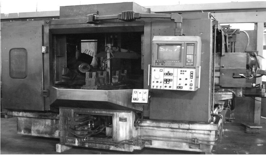
Goss & Deleeuw Twin Turret CNC Horizontal Machining Center, Fanuc 15 TT
