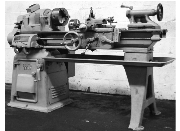
Southbend 12" x 30" Lathe
