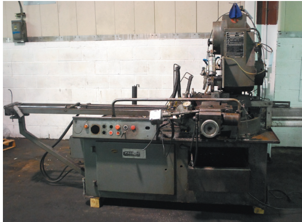
Tenn Jaeger #VC400HA, 16" Automatic Universal Cold Saw
