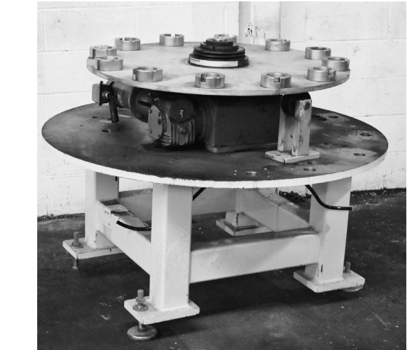
Ferguson 12 Station, 36" Rotary Index Table
