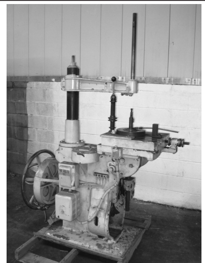
Baker #0 Keyseater CB 2604 $2,250
