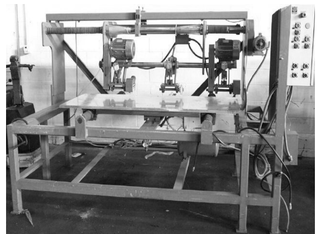
Mc Cormick 2' x 2' Panel Groover
