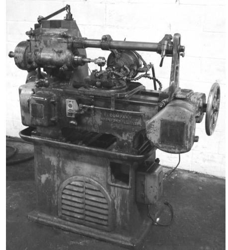
Barber Colman 6-10 Gear Hobber BR 8630 $2,450
