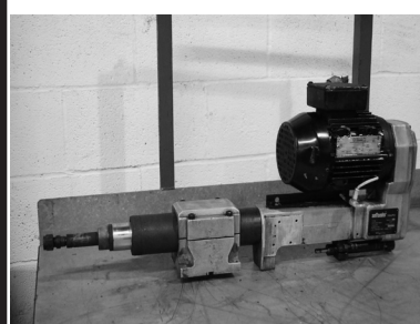
Sugino #SN4LU 1/2 HP Selffeeder Electric Drill $245 BR 8906
