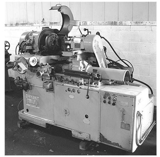
Bryant #1116 Internal Grinder
