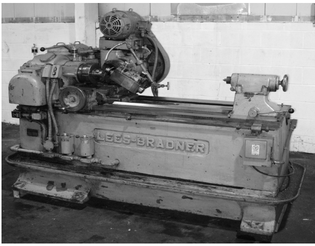
Lees - Bradner #HT 12" x 24" Thread & Worm Milling Machine MV 1098 $8,950
