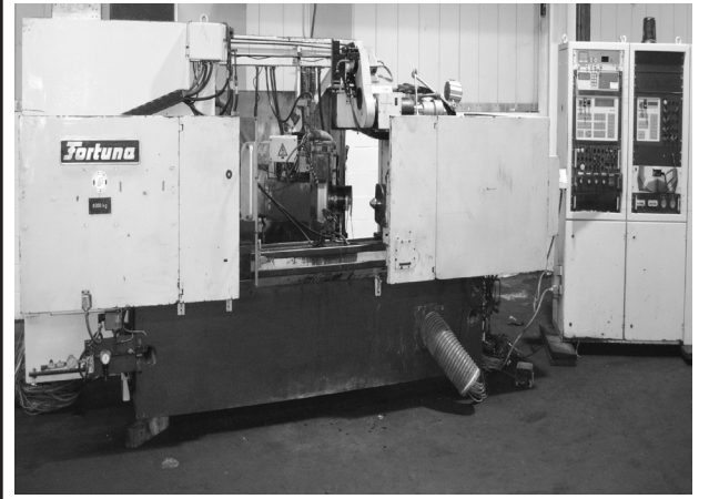
Fortuna #FM43, 13" x 44" Cnc Angle Head Cylindrical Grinder
