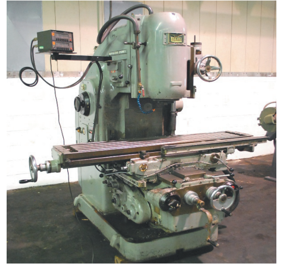
Hitachi Seiki #2ML-V Vertical Mill
