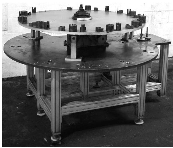
Ferguson 54" Rotary Index Table, 16 Position
