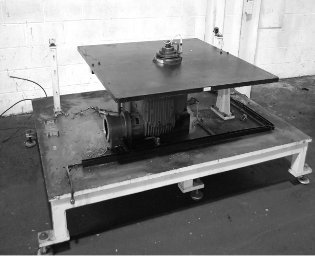
Ferguson 46" "Rotary Index Table, 2 Position
