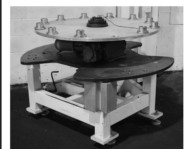
Ferguson 12 Station, 48" Rotary Index Table
